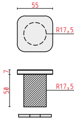
COPRIFORO PER LAVABO/BIDET TAP HOLE COVER FOR WASHBASIN/BIDET SATINATA – LUCIDA – CARBONE SATIN – CHROME – CARBON
