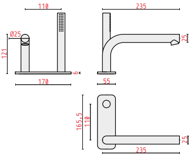
GRUPPO BORDOVASCA CON DOCCINO DECK-MOUNTED SPOUT FOR BATHTUB WITH HAND SHOWER
