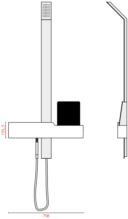
COLONNA DOCCIA ESTERNA CON TOUCH PANEL, SOFFIONE E DOCCINO EXTERNAL SHOWER COLUMN WITH HEAD SHOWER AND HAND SHOWER CONTROLLED BY TOUCH PANEL
