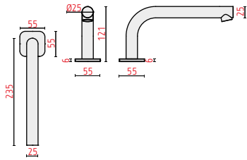
GRUPPO BORDOVASCA DECK-MOUNTED SPOUT FOR BATHTUB
